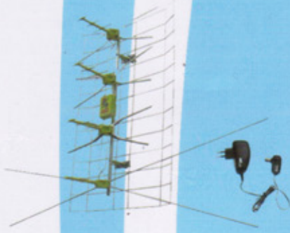
ASP-8B FREQUENCY RANGE: 47-862MHZ VHF/UHF GAIN: 15-28DB OUT IMPEDANCE: 75Ω STANDING WAVE RATIO(SWR): \leq 1.5 DB POWER SUPPLY: 12V/100MA ASSEMBLED WITH: AMPLIFIER SWA SERIES WEIGHT: 1,7 KG
