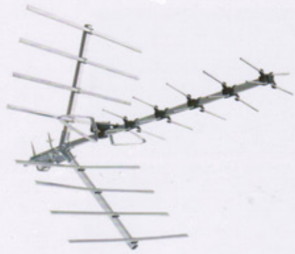
YG-032 FREQUENCY RANGE: 470-862MHZ RECEIVING RANGE: UHF GAIN: 18DB OUT IMPEDANCE: 75Ω STANDING WAVE RATIO: \leq 1.5 DB
