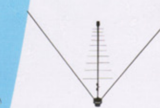
H311.01 FREQUENCY RANGE: 47-862MHZ VHF/UHF GAIN: 8DB CHANNEL 1-5 (VHF I 47-108MHZ): -0.5DB CHANNEL 6-12 (VHF II 174-230MHZ): 1DB CHANNEL 21-60 (UHF 470-862MHZ): 8DB OUT IMPEDANCE: 75Ω STANDING WAVE RATIO(SWR): ≤1.5DB WEIGHT: 1.6 KG
