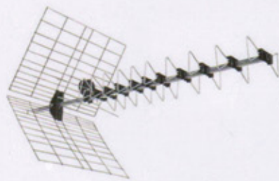
YG-056 FREQUENCY RANGE: 470-862MHZ RECEIVING RANGE: UHF GAIN: 18DB OUT IMPEDANCE: 75Ω STANDING WAVE RATIO(SWR): \leq 1.5 DB
